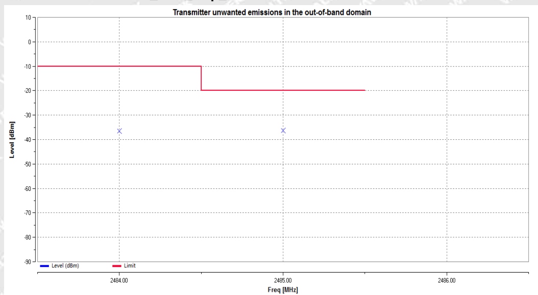
OOB_DH5_Hop_2483.5MHz to 2483.5MHz+2BW
