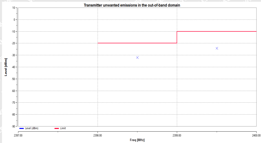
OOB_DH5_Hop_2400MHz-2BW to 2400MHz
