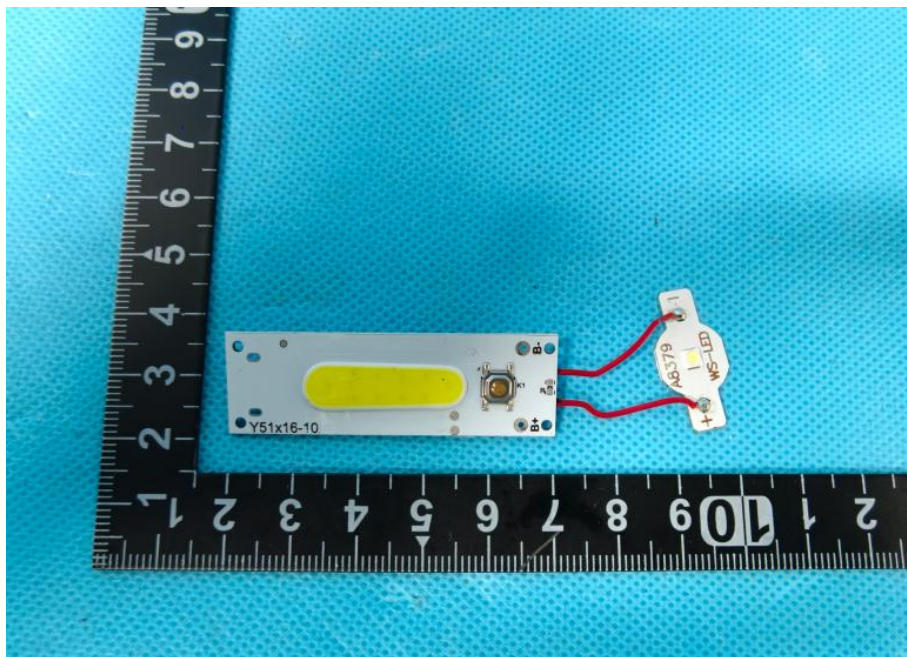
Fig.6 – Parts view
