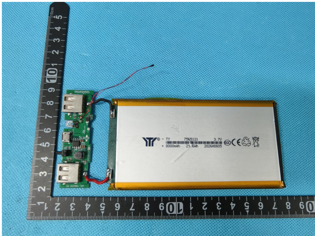
Fig. 8- Internal view
