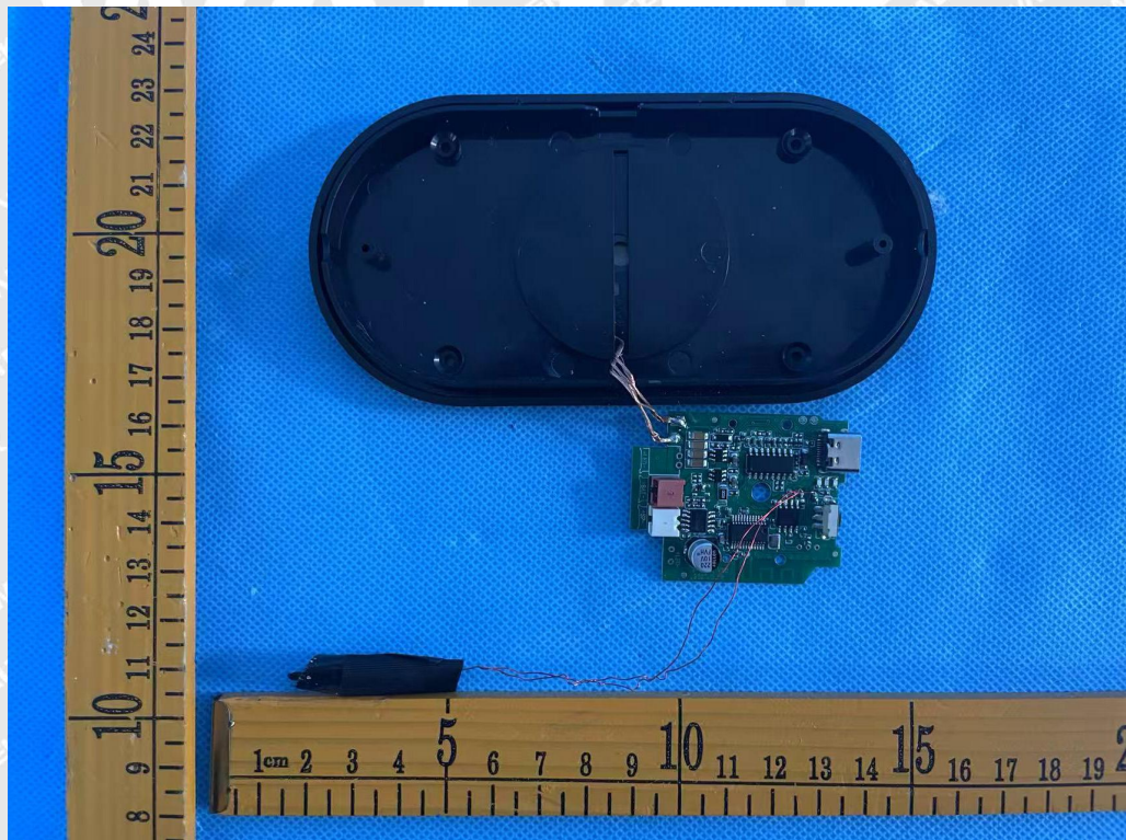
Figure 8 PCB view
