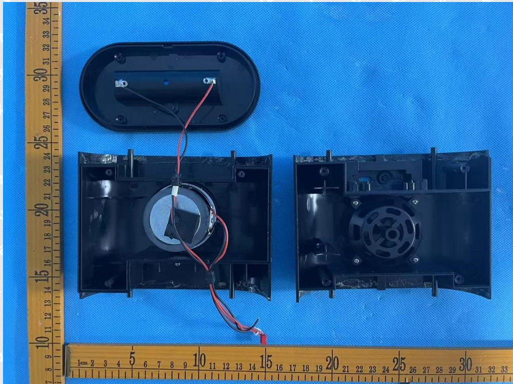
Figure 7 Internal view
