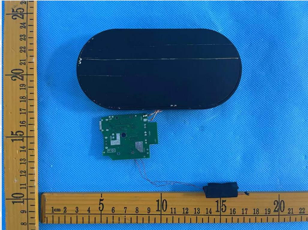
Figure 9 PCB view
