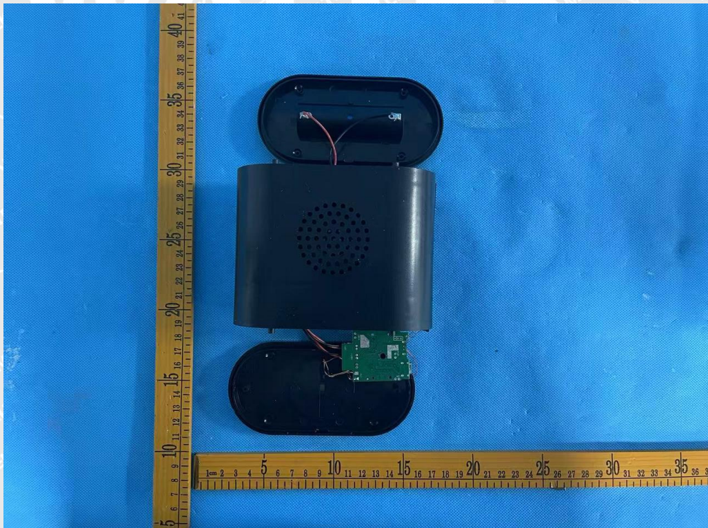
Figure 6 Internal view
